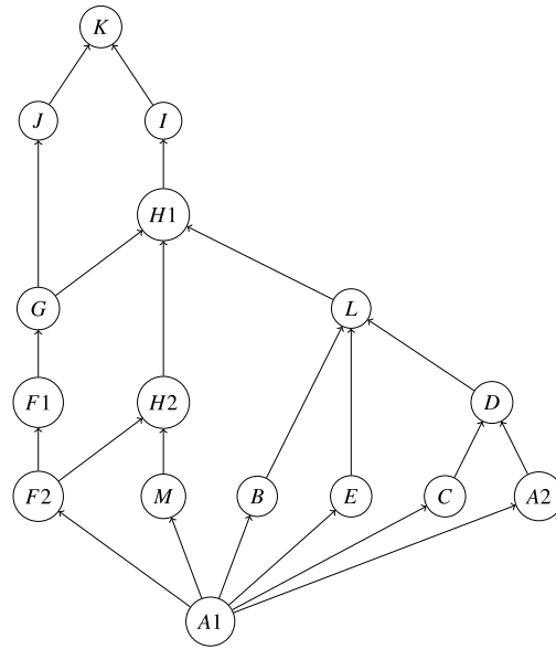
Fig. 2. Lattice of the fuzzy neighborhood operators from Table 2.
