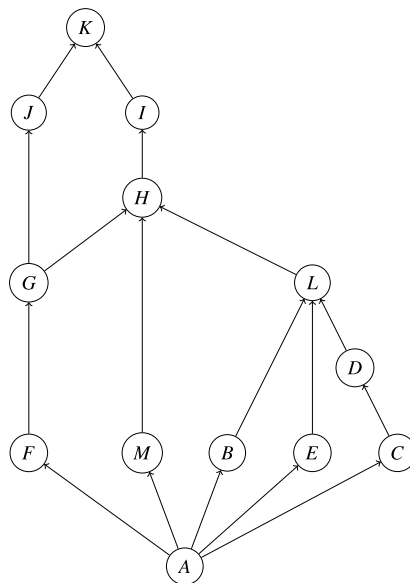
Fig. 1. Lattice of the neighborhood operators from Table 1.
