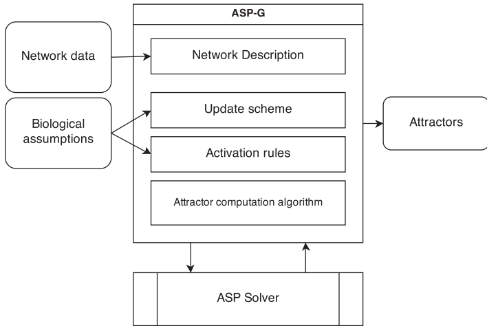
Fig. 2: Architecture of ASP-G.
